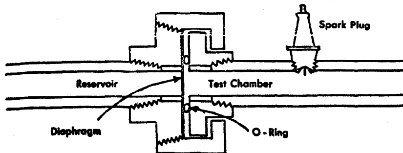
FIG 4 DIAPHRAGM ASSEMBLY
